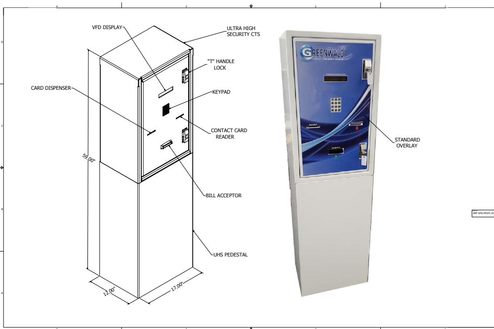
High Security Cash Box Drawing - Value station and Pedestal
